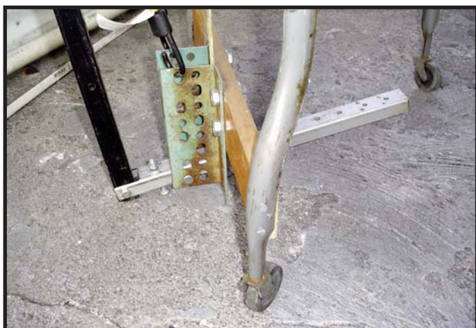
Figure 3. The treadle is made from a 15 inch piece of 3/4 inch by 1 1/4 inch steel channel. The pivot is located four inches from the rear end. The vertical bolt through the treadle provides an adjustable down-stroke stop.
